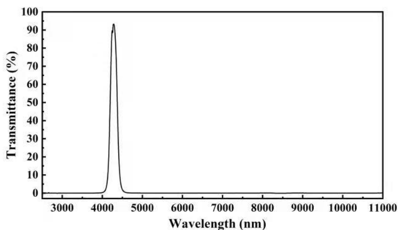
Transmittance of 4.26 \mu m Filter
