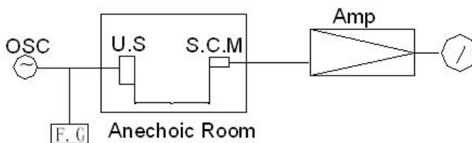
Transmitter
