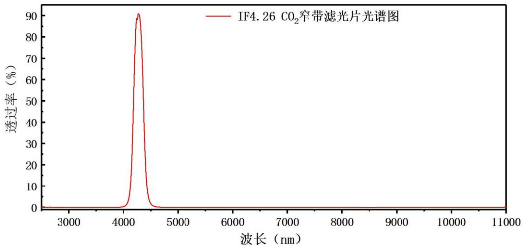
Transmittance of 4.26 \mu\text{m} Filter
