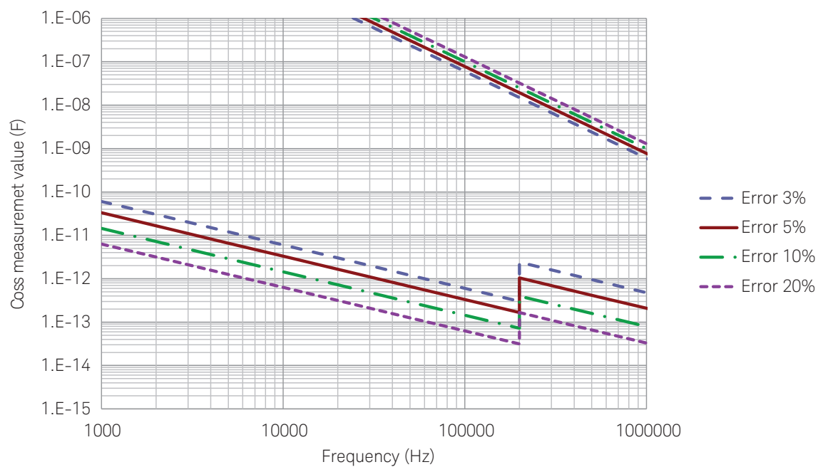
Coss measurement accuracy 3-terminal Cgs:Cds:Cgd = 1:0.1:0.01
