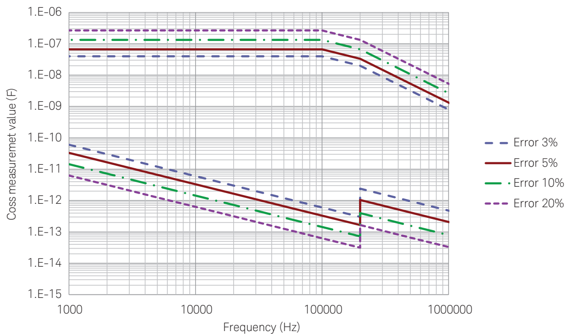
Coss measurement accuracy 3-terminal Cgs:Cds:Cgd = 1:1:1
