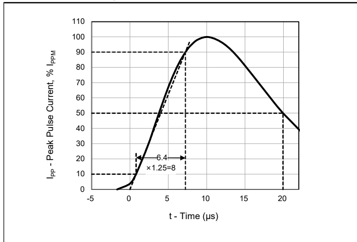
Fig.3 - 8/20 \mu s Pulse Waveform
