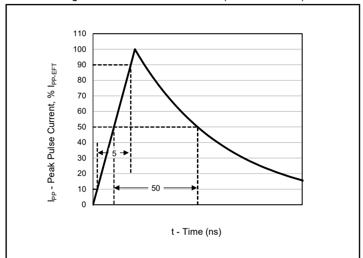
Fig.6 - 5/50ns EFT Waveform (IEC61000-4-4)
