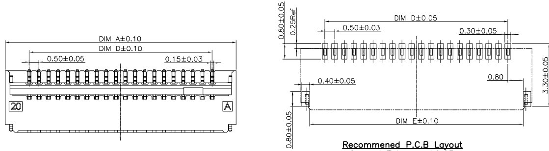
Recommended P.C.B Layout General Tolerance ±0.05
