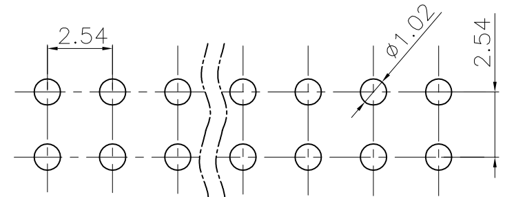
RECOMMENDED PCB LAYOUT TOLLERANCE: ±0.05
