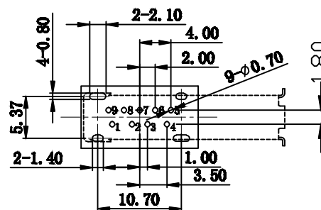
Recommended P.C.B Layout General Tolerance±0.05 TOP VIEW
