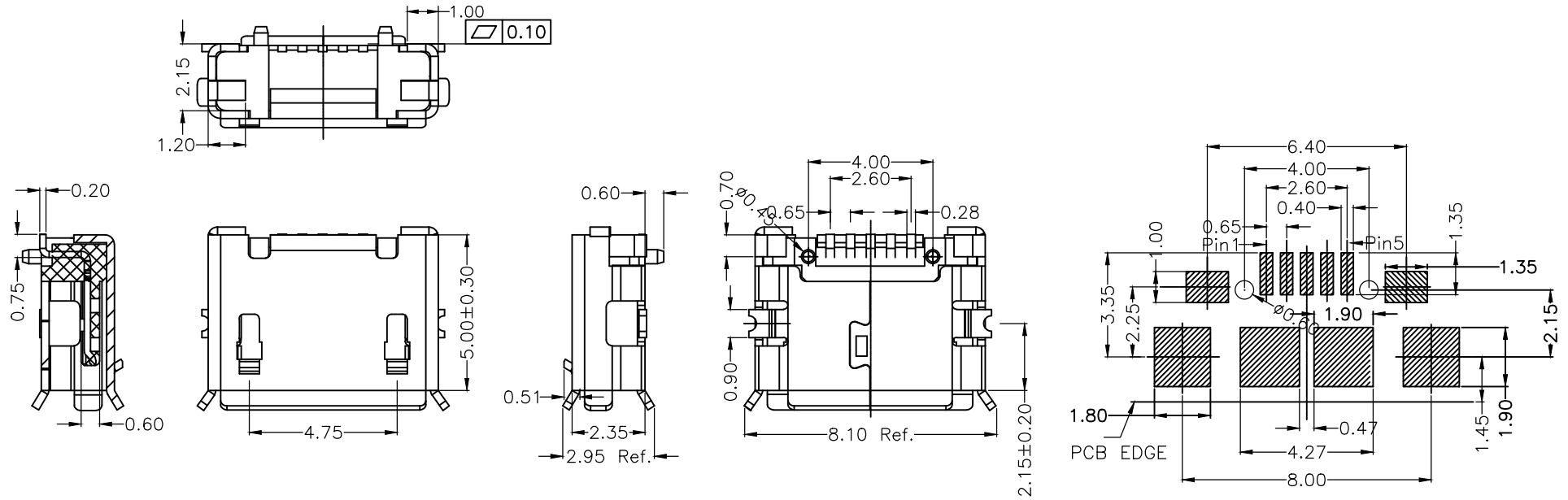
RECOMMENDED PCB LAYOUT PCB图仅供参考
