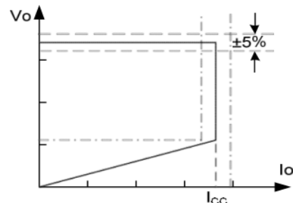
Fig.1. Typical CC/CV Curve
