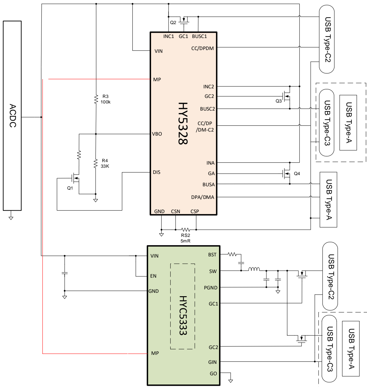
Fig. 8. Regulation the VIN voltage Application
