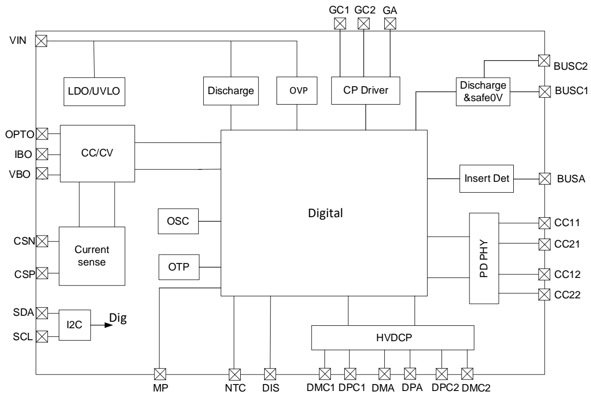
Fig. 3. Function Block
