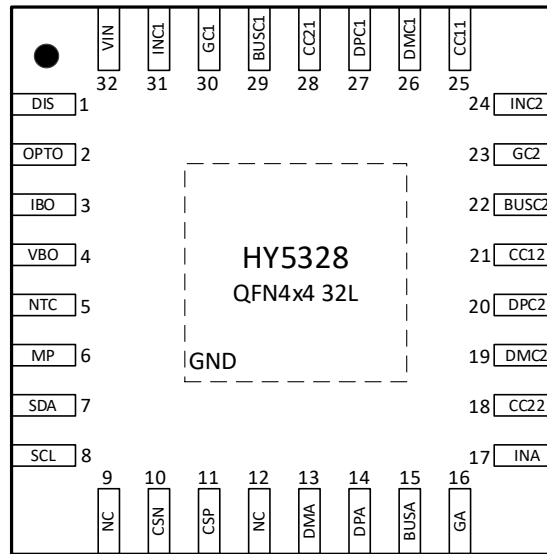
QFN 4mm x 4mm - 32L
