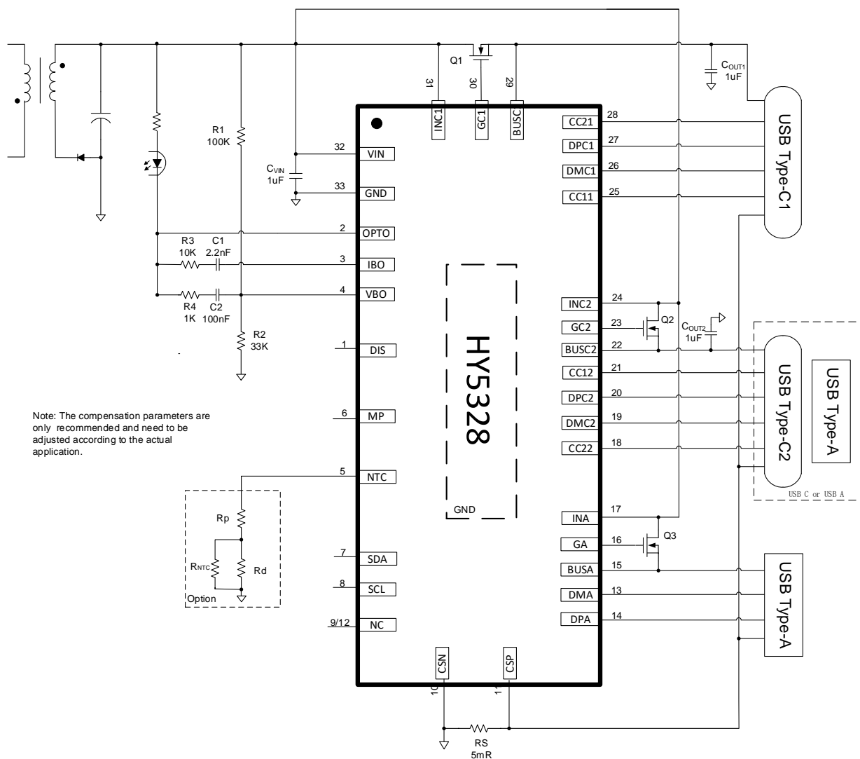
Fig. 6. 2C1A or 1C2A Application for OPTO feedback
