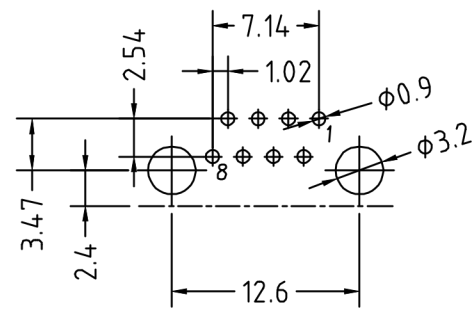
SUGGESTED PCB LAYOUT (TOP VIEW)
