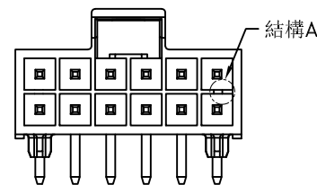
GJS-2513RA-XXx2 Color: Black
