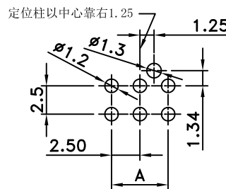
Recommended PCB Layout (06 & 10 & 14) General Tolerance ±0.05
