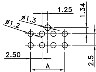
Recommended PCB Layout (04 & 08 & 12 & 16) General Tolerance ±0.05
