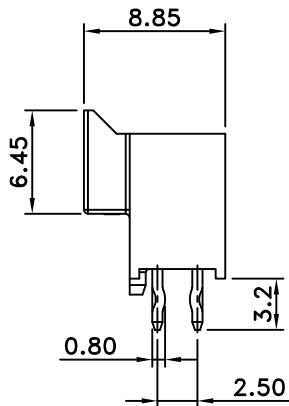
GJS-2513A-XXx2 Colour: Black
