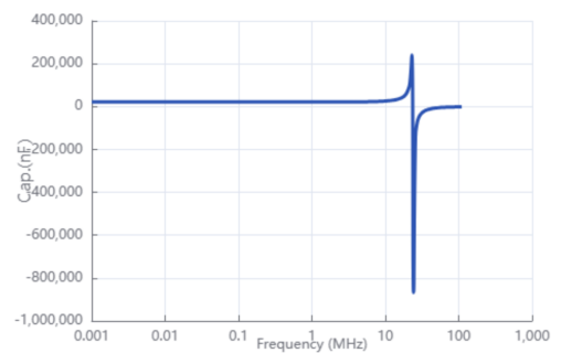
Capacitance-Frequency
