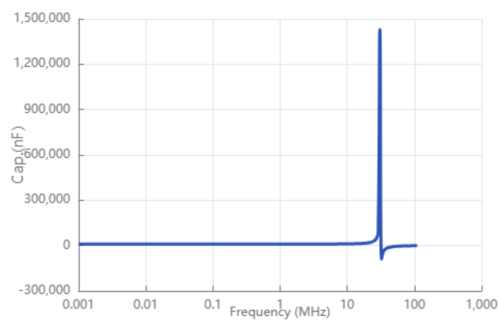
Capacitance-Frequency
