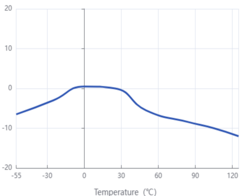
Capacitance-Temperature Characteristics
