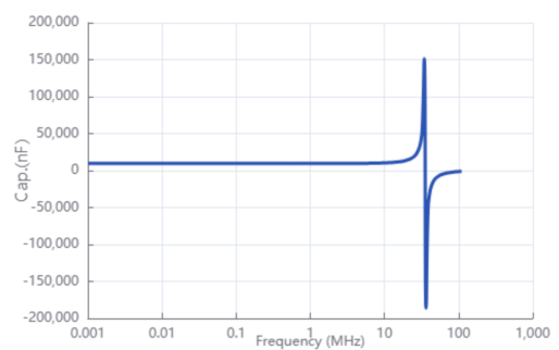
Capacitance-Frequency
