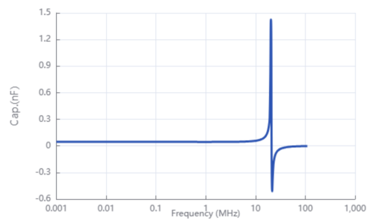
Capacitance-Frequency
