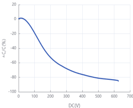
Capacitance-DC Voltage Characteristics
