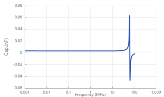
Capacitance-Frequency
