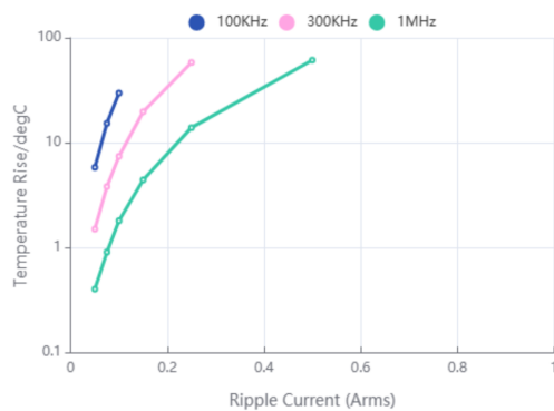
Temperature Rise-Ripple Current
