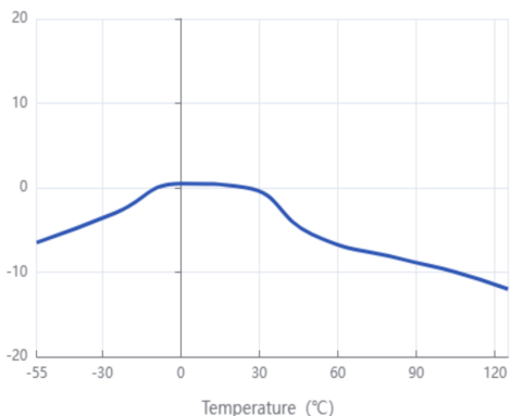
Capacitance-Temperature Characteristics
