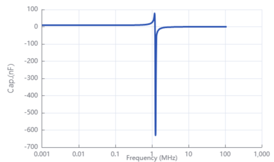
Capacitance-Frequency
