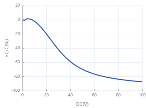
Capacitance-DC Voltage Characteristics
