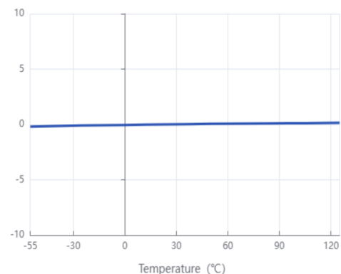
Capacitance-Temperature Characteristics
