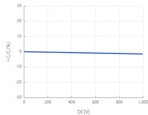
Capacitance-DC Voltage Characteristics
