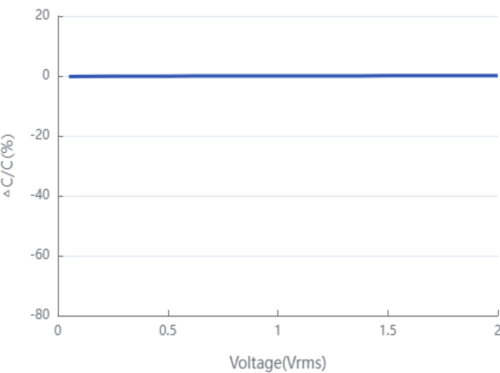
Capacitance-AC Voltage Characteristics
