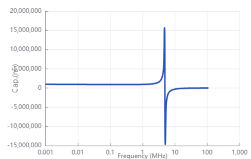
Capacitance-Frequency
