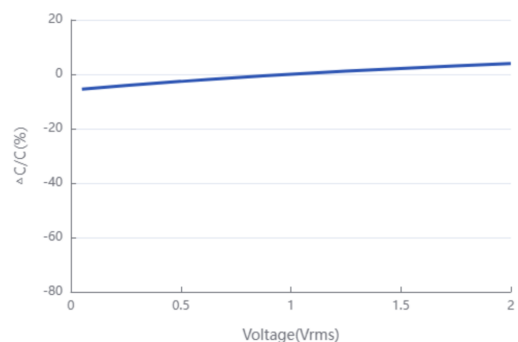
Capacitance-AC Voltage Characteristics
