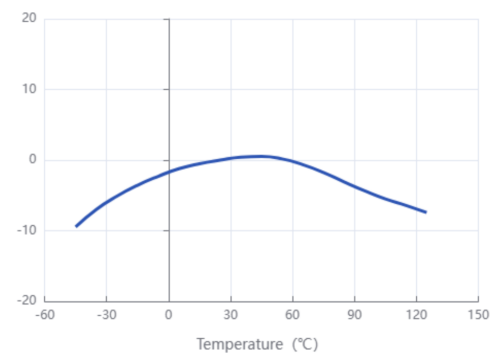
Capacitance-Temperature Characteristics
