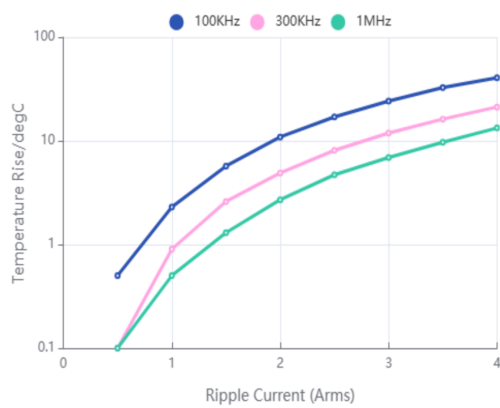
Temperature Rise-Ripple Current
