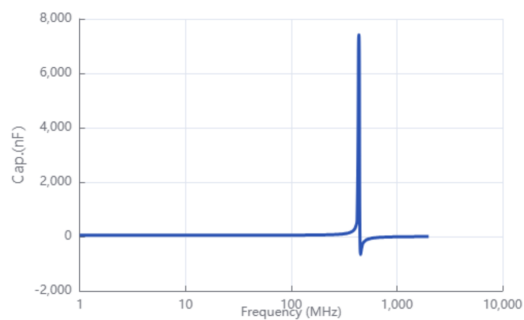
Capacitance-Frequency
